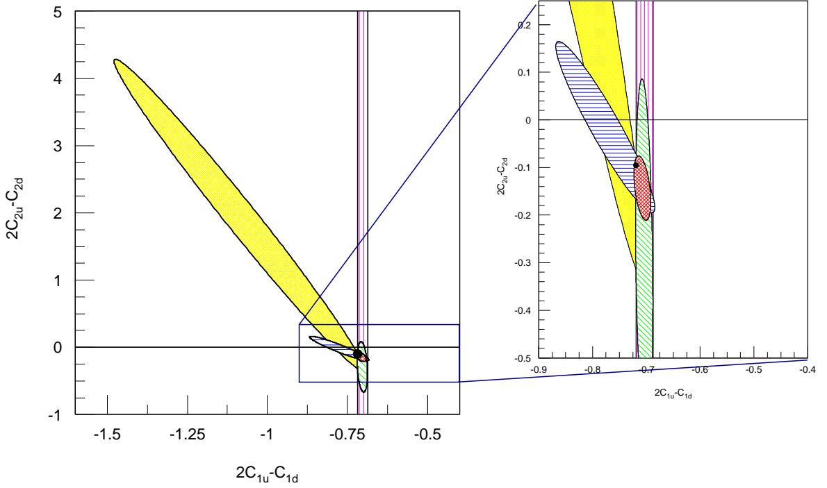
FIG. 23: From Ref. [48]: results on (2C_{1u} - C_{1d})|_{Q^2=0} and (2C_{2u} - C_{2d})|_{Q^2=0} from the present experiment. The right panel shows an enlarged view with the vertical and the horizontal axis at the same scale. The new results (blue horizontal-line-hatched ellipse) are compared with SLAC E122 (yellow ellipse) [8, 9]. The latest data on C_{1q} [31] (from PVES and Atomic Cs [32–35]) are shown as the magenta vertical-line-hatched band. The green slanted-line-hatched ellipse shows the combined result of SLAC E122 and the latest C_{1q} , while the red line-cross-hatched ellipse shows the combined result of SLAC E122, the present experiment, and the latest C_{1q} . The Standard Model value 2C_{2u} - C_{2d}|_{Q^2=0} = -0.0950 \pm 0.0004 is shown as the black dot, where the size of the dot is for visibility.
