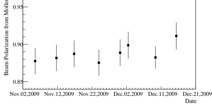
FIG. 9: Polarization results from the Møller polarimeter measurements taken with a beam energy of 6.067 GeV. The error bars represent the quadratic sum of the statistical and systematic errors. However, for each measurement the statistical uncertainty was in the order of 0.1%, much smaller than the systematic error. An additional measurement was done with a beam energy of 4.867 GeV at the end of the run period, which gave a similar polarization.
