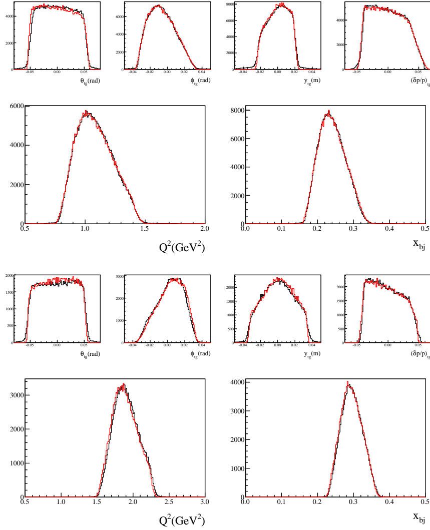
FIG. 15: Comparison between HAMC (red) and data (black). From top to bottom: target variables -\theta_{t\bar{g}}, \phi_{t\bar{g}}, y_{t\bar{g}} and (\delta p/p)_{t\bar{g}} – for Left HRS DIS#1; Q^2 and x for Left HRS DIS#1; target variables for Right HRS DIS#2; Q^2 and x for Right HRS DIS#2.
