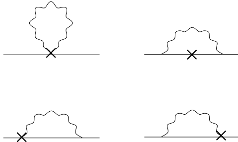
FIG. 3: One-loop diagrams contributing to the fermion-antifermion Green's functions of the bilinear operators. A wavy (solid) line represents gluons (fermions). A cross denotes an insertion of the operator \mathcal{O}_\Gamma .
