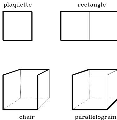
FIG. 1: The four Wilson loops of the gluon action.
