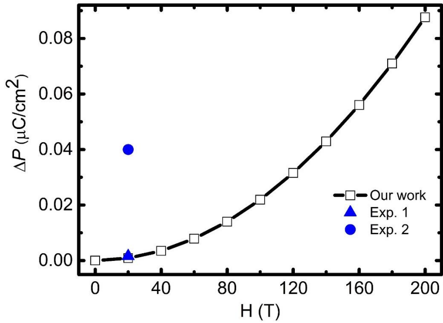
Figure 4. Polarization (P) versus magnetic field (H) calculated from our simple theoretical model. \Delta P is defined as \Delta P = P(H) - P(0) . Experimental results (Exp.1 [32] and Exp. 2 [33]) are also shown for comparison.
