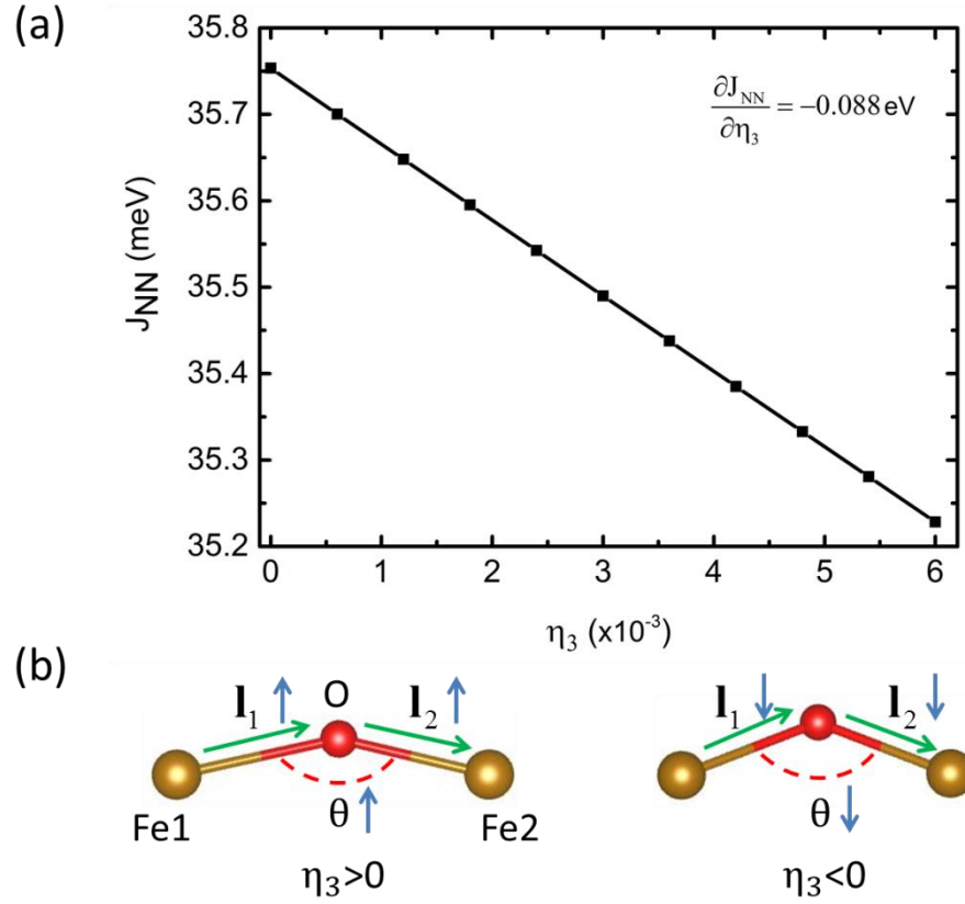
Figure 3. (a) The NN symmetric spin exchange interaction J_{NN} as a function of \eta_3 . The obtained
