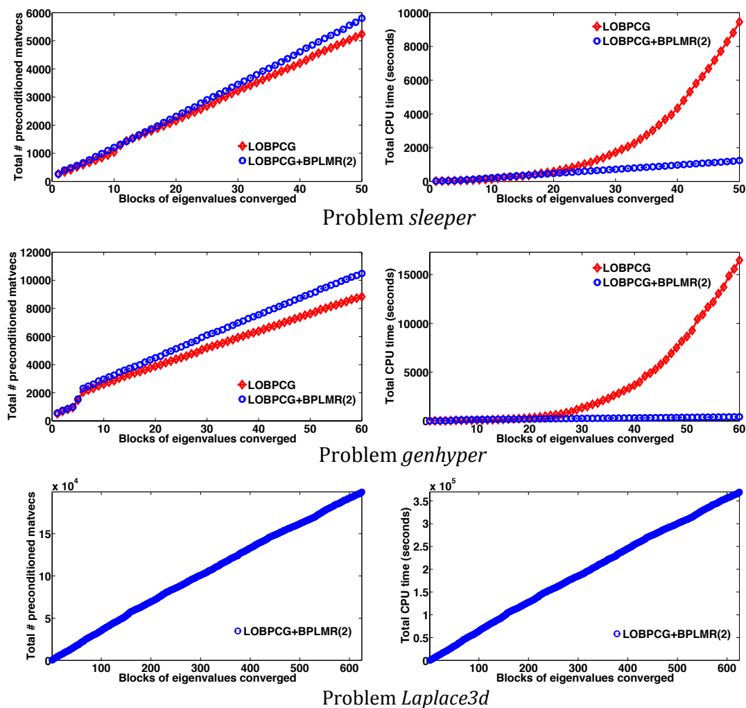
FIG. 6.1. Total number of preconditioned matrix-vector products and CPU time used by LOBPCG and LOBPCG+BPLMR(2). Top: sleeper , lowest 500 eigenvalues Medium: genhyper , highest 600 eigenvalues Bottom: Laplace3d , lowest 10002 eigenvalues (only LOBPCG+BPLMR(2) is used)
