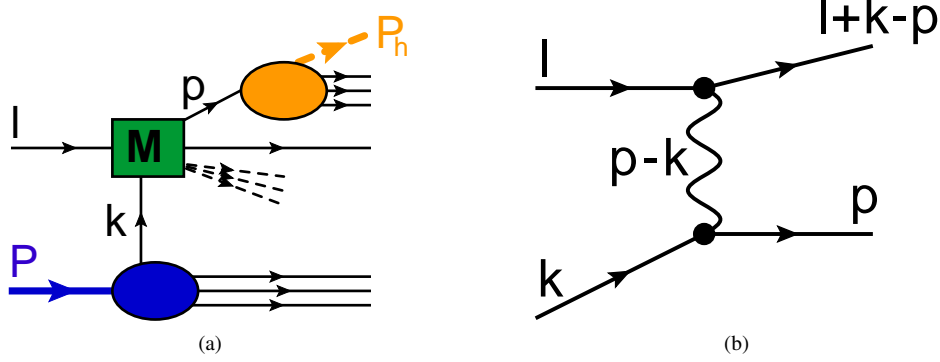
FIG. 1. Subfigure (a): Factorization (of the amplitude) in terms of two-parton quark correlators of the process \ell(l) + N(P) \rightarrow h(P_h) + X . The square blob stands for the hard partonic scattering while the bottom and top oval blobs represent the soft distribution and fragmentation functions, respectively. This diagram describes twist-2 observables and intrinsic and kinematical twist-3 effects. Subfigure (b): Leading-order diagram for the hard partonic scattering.
