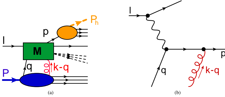
FIG. 2. Subfigure (a): Factorization (of the amplitude) in terms of quark-gluon-quark correlators for distributions. The square blob stands for the hard partonic scattering while the bottom oval blob represents the three-parton distribution functions, and the top oval blob represents a twist-2 fragmentation. This diagram describes dynamical twist-3 effects. Subfigure (b): Leading-order diagram for the hard partonic scattering.
