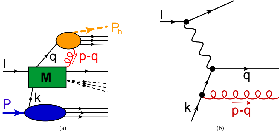
FIG. 3. Subfigure (a): Factorization (of the amplitude) in terms of quark-gluon-quark correlators for fragmentation. The square blob stands for the hard partonic scattering while the top oval blob represents the three-parton fragmentation functions, and the bottom oval blob represents a twist-2 parton distribution. This diagram describes dynamical twist-3 effects. Subfigure (b): Leading-order diagram for the hard partonic scattering.
