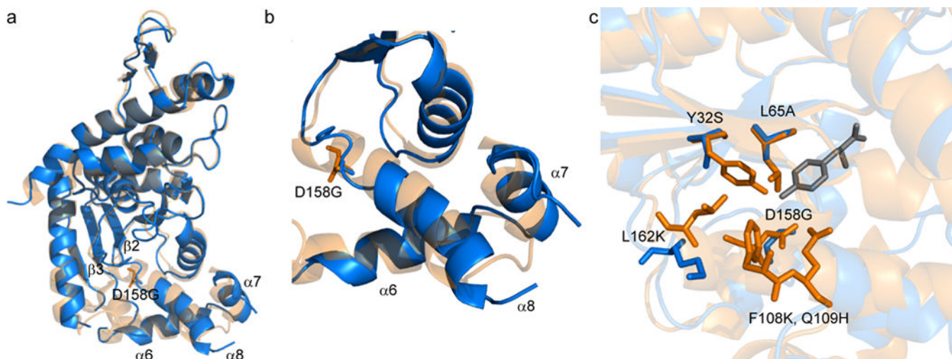
Figure 4. X-ray structure of CMFRS
