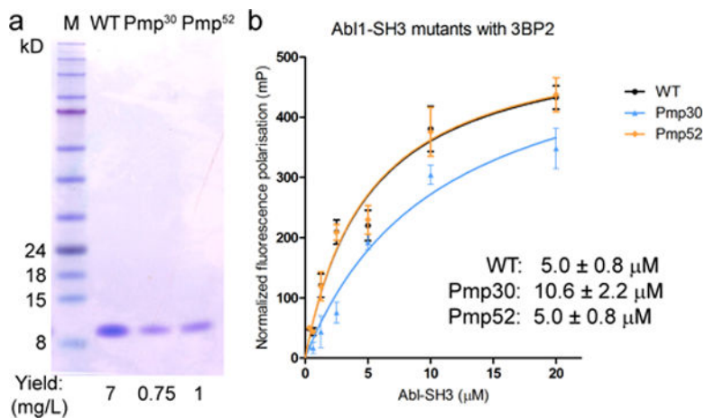
Figure 3. Expression and characterization of human Abl1 and its Pmp-containing variants in E. coli
