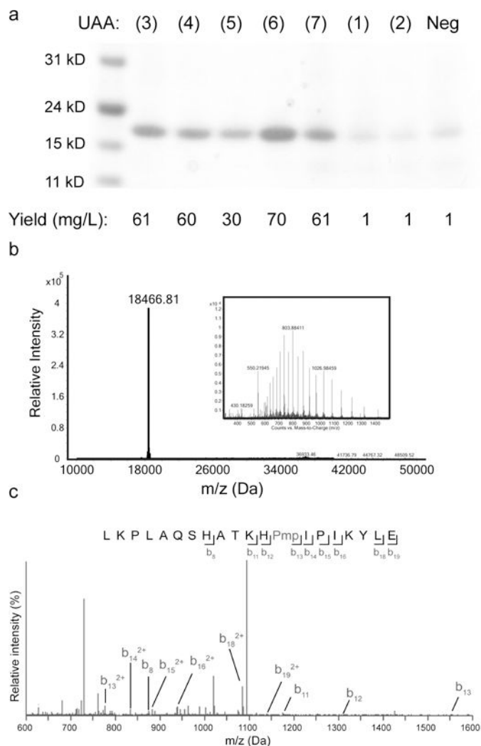
Figure 2. Incorporation and characterization of variant myoglobins containing different ncAAs (a) SDS-PAGE analysis of Myo-K99TAG expressed with CMFRS in the presence or absence of various ncAAs or dipeptides and stained with Coomassie blue (full gel image in Supplementary Fig. 1). (b) Deconvoluted mass spectrum of Myo-K99Pmp; inset, mass spectrum before deconvolution. (c) MS/MS fragmentation of GluC-digested peptides derived from Myo-K99Pmp. The spectrum confirmed that Pmp had been incorporated at the desired site.
