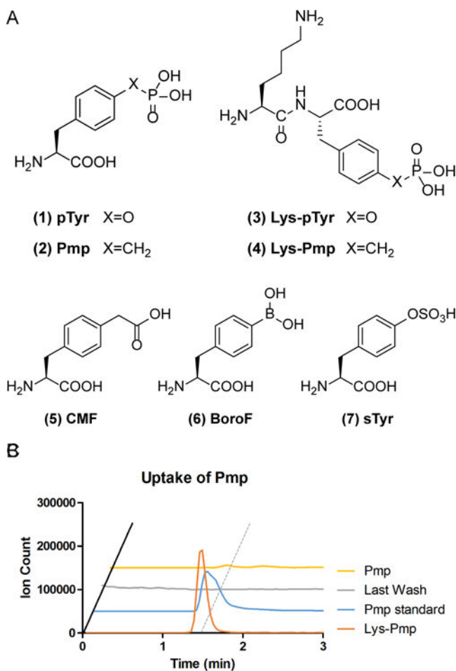
Figure 1. Pro-peptide strategy to increase the intracellular concentrations of pTyr and Pmp (a) Structures of ncAAs used in this study. (b) The extracted-ion chromatogram for uptake of Lys-Pmp. 5 mM Lys-Pmp (orange) or Pmp (yellow) was added during incubation. Blue, 50 \mu M Pmp was added to the cell lysate as standard; gray, buffer from last wash before cell lysis.
