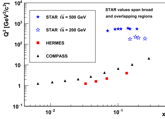
Fig. 1. Q^2 vs x coverage for STAR, HERMES, and COMPASS [13–17]. The kinematics of the STAR data points correspond to the lower panel of Fig. 3.
