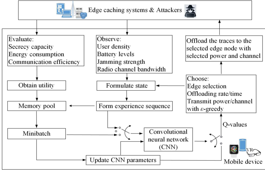
Fig. 3. Illustration of the DQN-based secure offloading in mobile edge caching.
