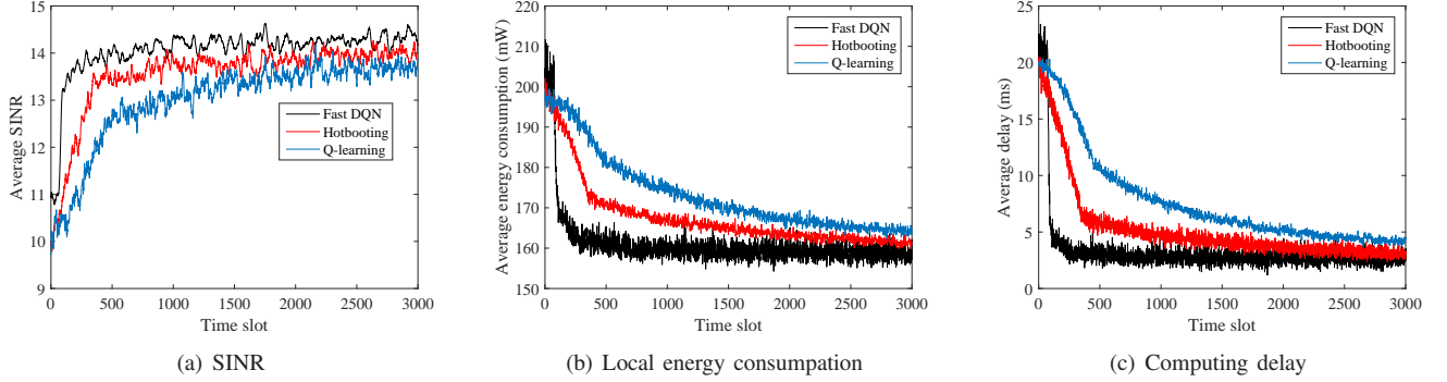
Fig. 4. Performance of the RL-based offloading for a mobile device that is close to 3 edge devices against jamming.
