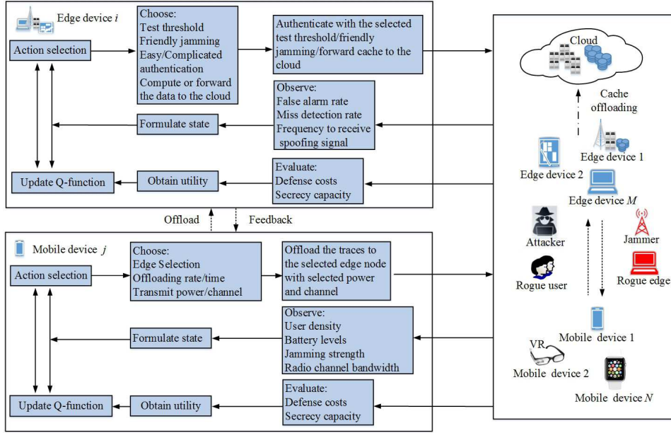
Fig. 2. RL-based security solutions for MEC systems.
