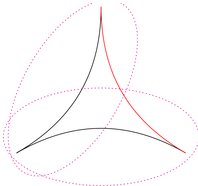
Figure 2.5: Gromov's thin triangle condition
