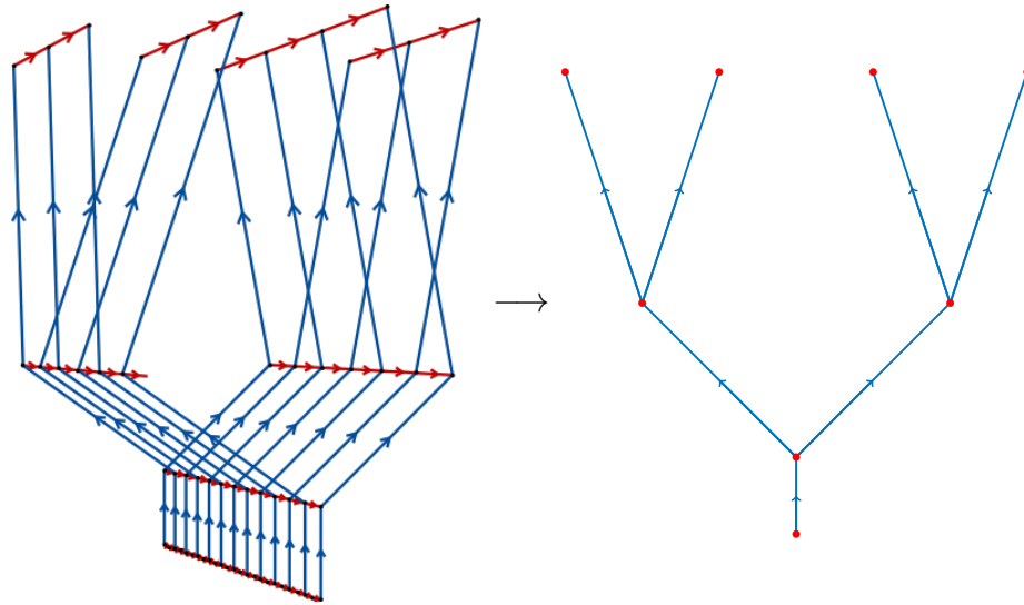
Figure 2.6: The Baumslag–Solitar group BS(1, m) has exponential growth
