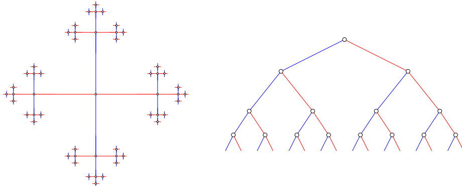
Figure 1.1: Exponentially growing Cayley graphs
