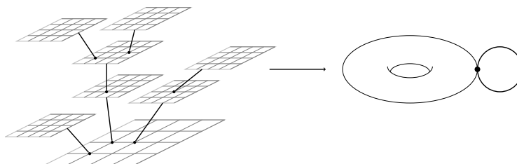
Figure 3.4: Universal cover of the Salvetti Complex of \mathbb{Z}^2 * \mathbb{Z}
