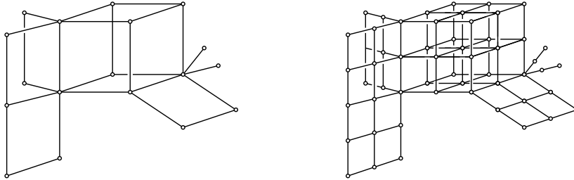
Figure 3.3: An example of cubical subdivision
