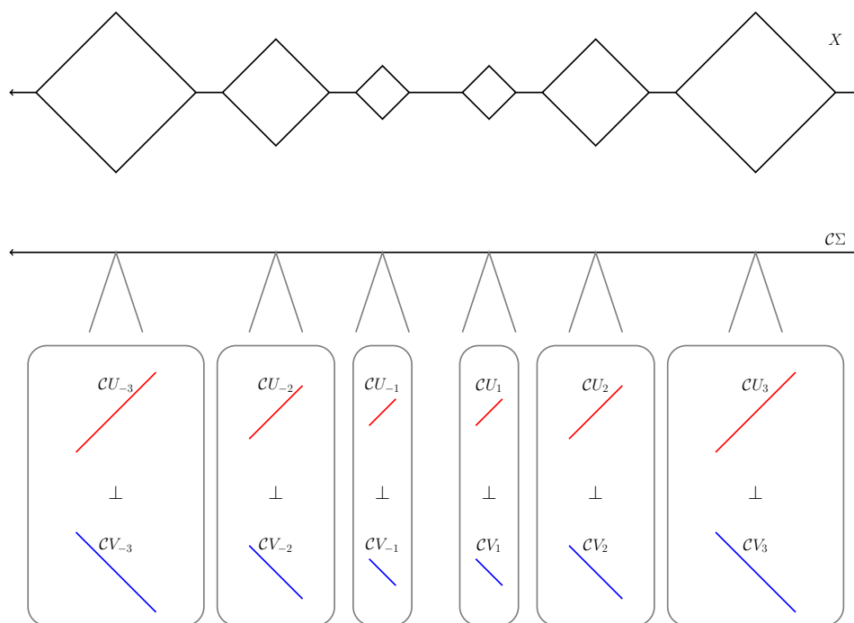
Figure 4.1: The real line where each integer n has been replaced by an n \times n square admits a hierarchically hyperbolic structure that does not satisfy the bounded domain dichotomy
