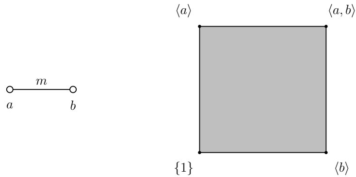
Figure 3.6: Fundamental domain of the Deligne complex
