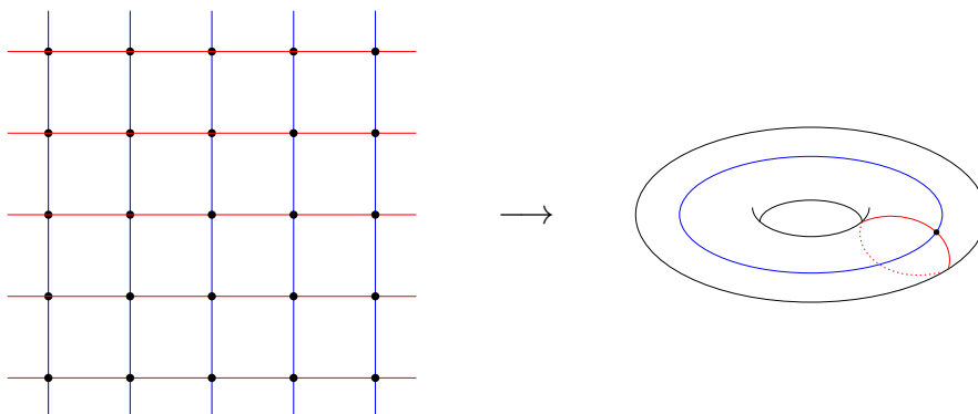
Figure 2.2: Presentation 2-complex of \mathbb{Z}^2
