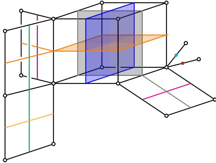
Figure 3.5: Hyperplanes in a cube complex
