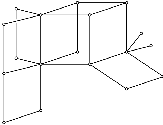
Figure 3.1: An example of a CAT(0) cube complex
